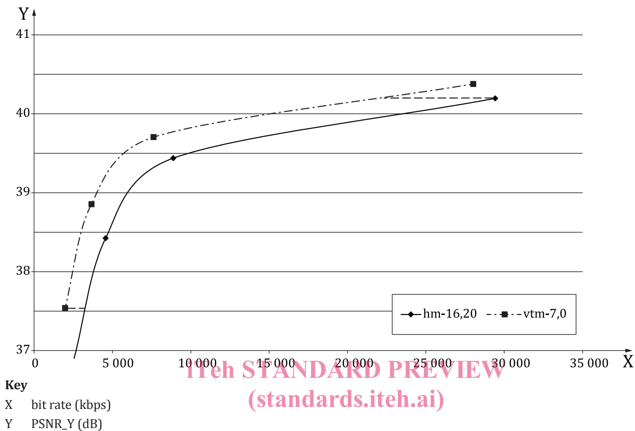
Figure 1 — Example of luma PSNR plotted as a function of bit rate for HM-16.20 (unbroken line) versus VTM-7.0 (dashed-dotted line)
