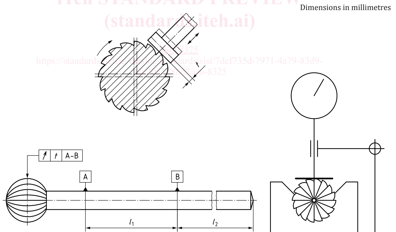
Figure 1 — Example of a V-block measuring device
