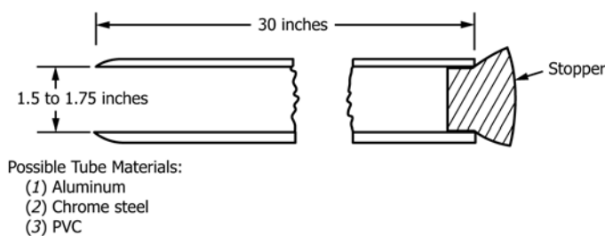
FIG. 1 Sampling Tube
