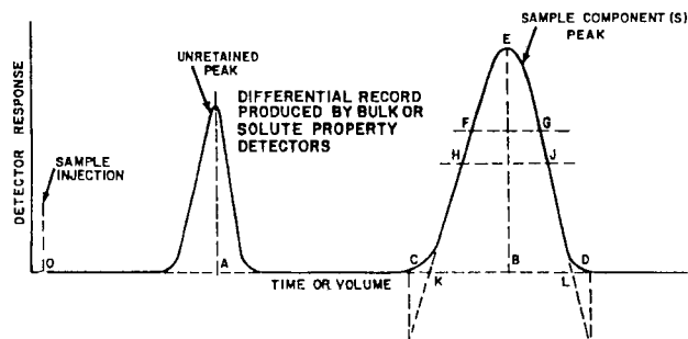
FIG. 2 Typical Chromatogram
