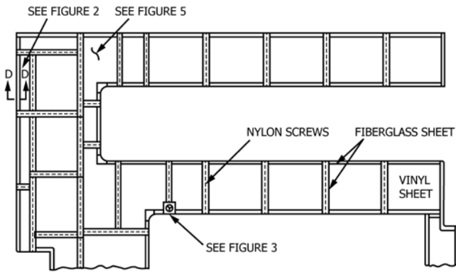
FIG. 1 Typical Deck Covering Plan View
