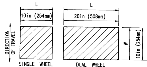
FIG. 3 Wheel Load Area
