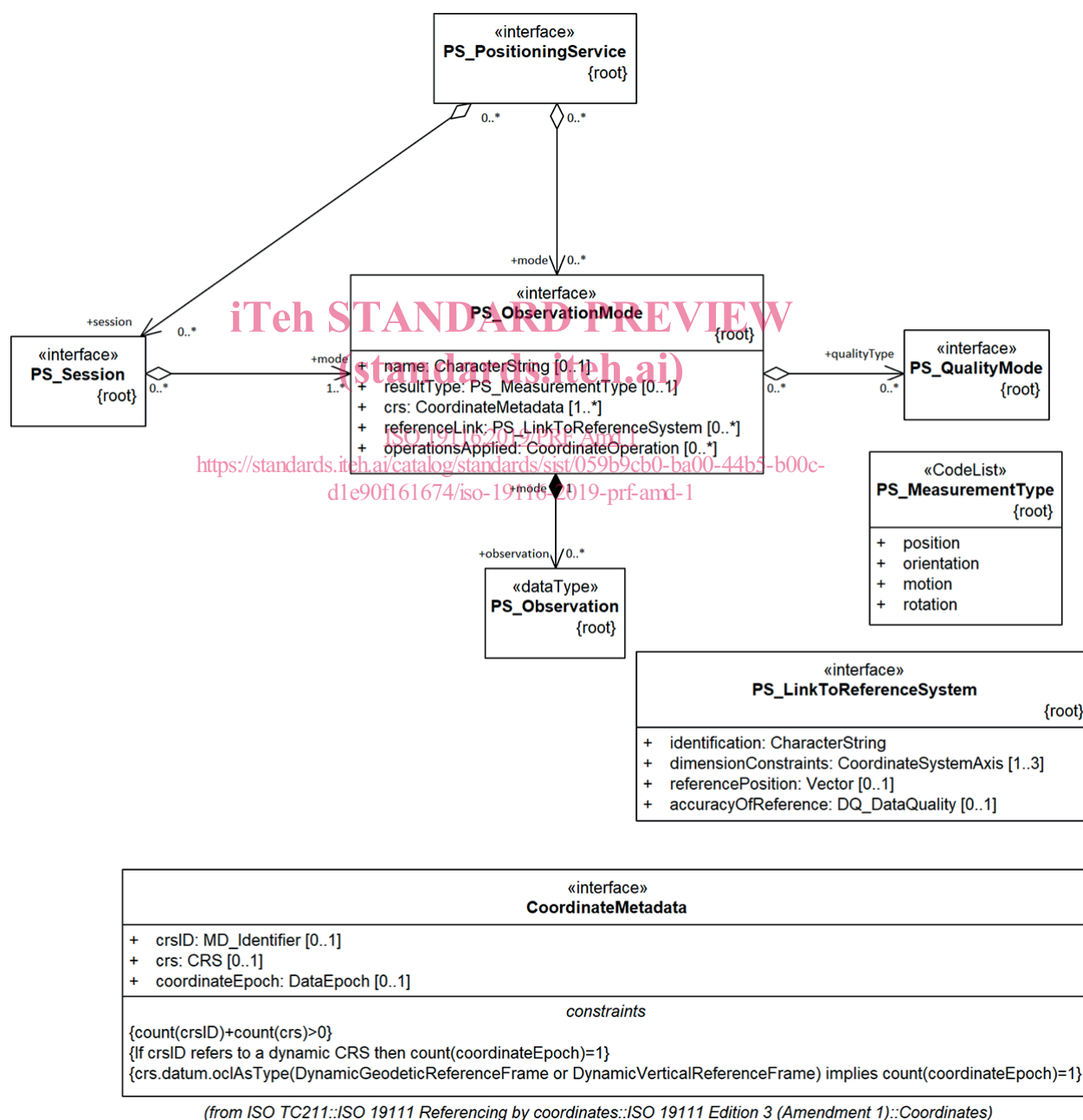
Figure 6 — UML diagram — PS_ObservationMode class and related data types
