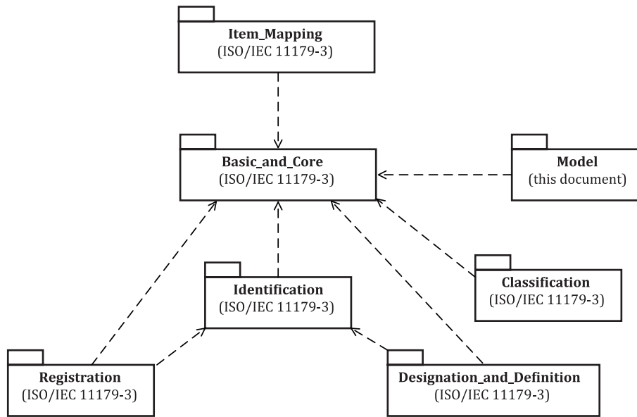
Figure 1 — Package dependencies
