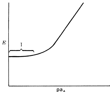
FIG. 1 Limit of Detection Example Response Curve (log activity on the horizontal axis)
