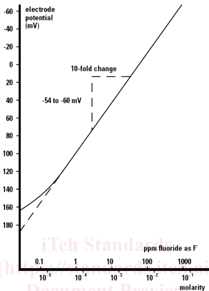
FIG. 2 Practical Limit of Detection Example Calibration Curve (log concentration on the horizontal axis)
