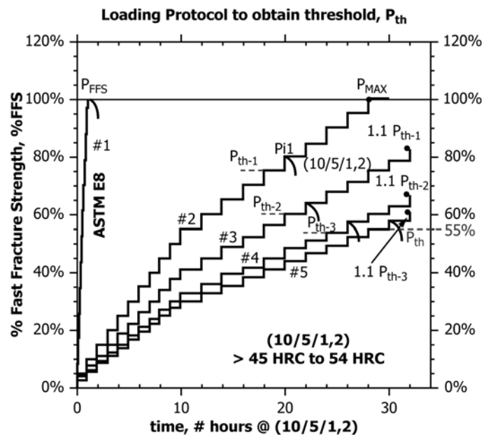
FIG. 2 Schematic of a (10/5/1,2) Step Loading Profile to Determine Threshold for the Hardness of Steel >45 HRC to 54 HRC
