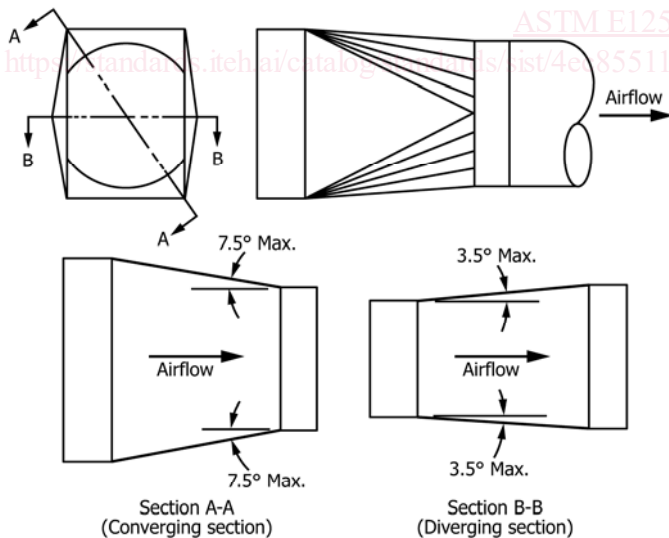
FIG. 4 Transformation Piece
