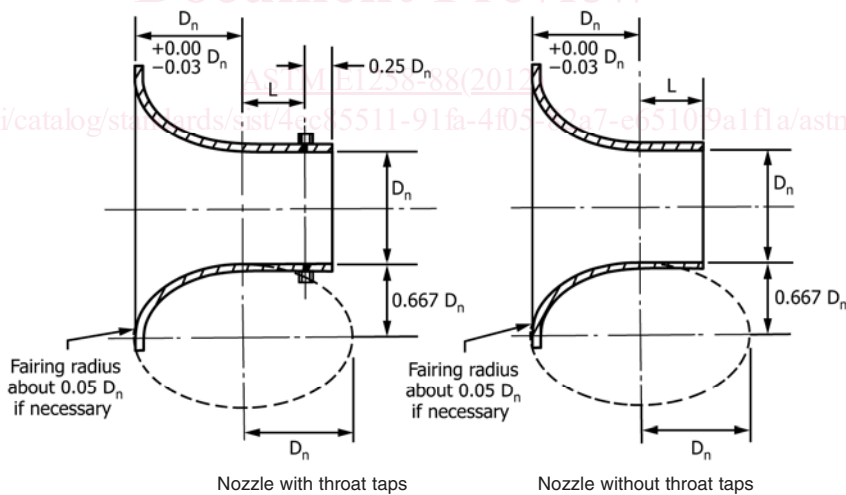
Nozzle with throat taps
