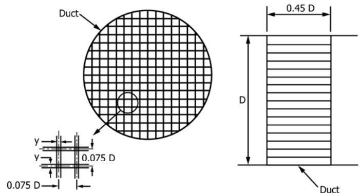
FIG. 6 Flow Straightener Specifications
