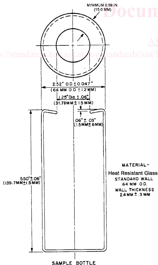
FIG. 3 Sample Bottle
