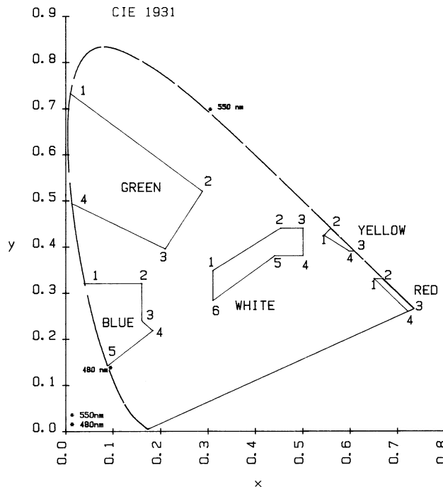
FIG. 1 Color Gamut in accordance with 6.2.4
