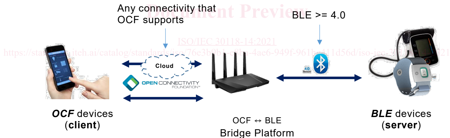
Figure 2 – BLE Bridging use case in real life
