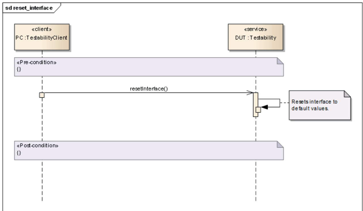
Figure 4 — Method resetInterface()
