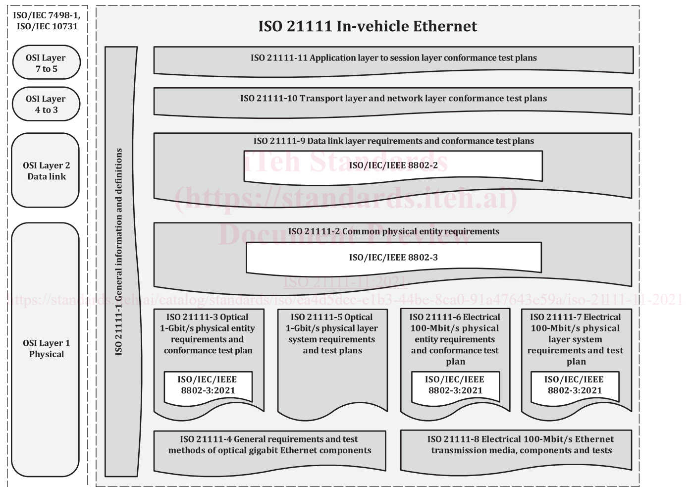
Figure 1 — In-vehicle Ethernet documents reference according to OSI model
