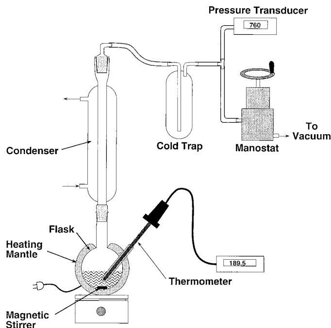
FIG. 2 Stirred-Flask Ebulliometer
