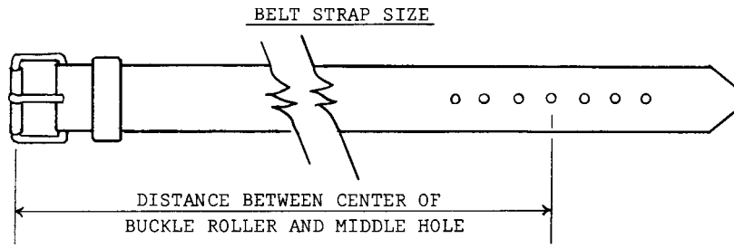
FIG. 13 Body Belt Strap Size
