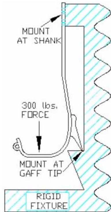
FIG. 5 Fatigue Test Fixture
