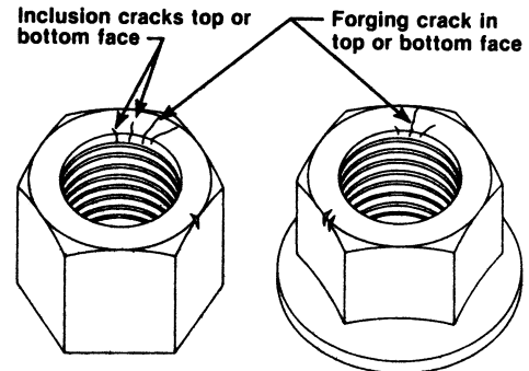
FIG. 2 Typical Forging and Inclusion Cracks in Nuts
