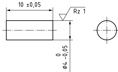
Figure 3 — Test cylinder for magnet efficiency
