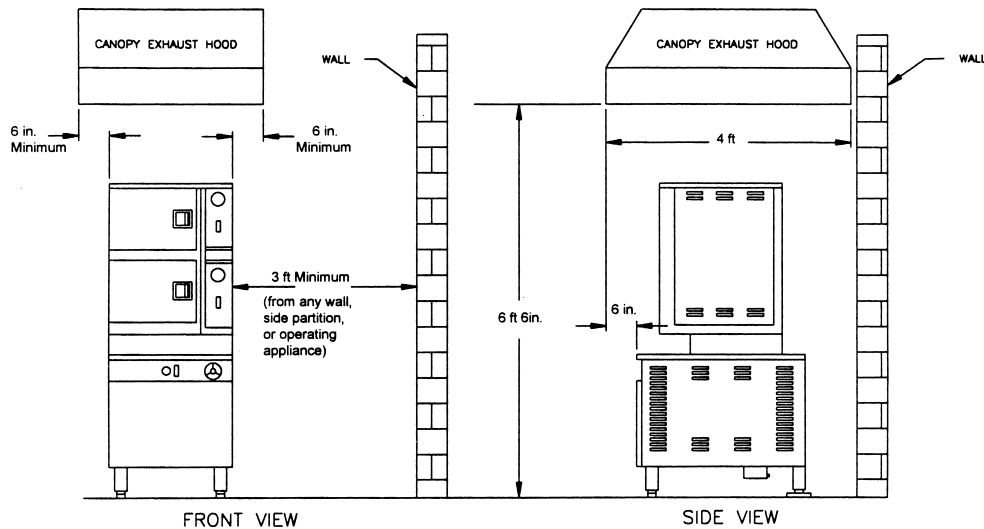
FIG. 3 Equipment Configuration
