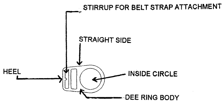
FIG. 1 Typical Dee-Ring
