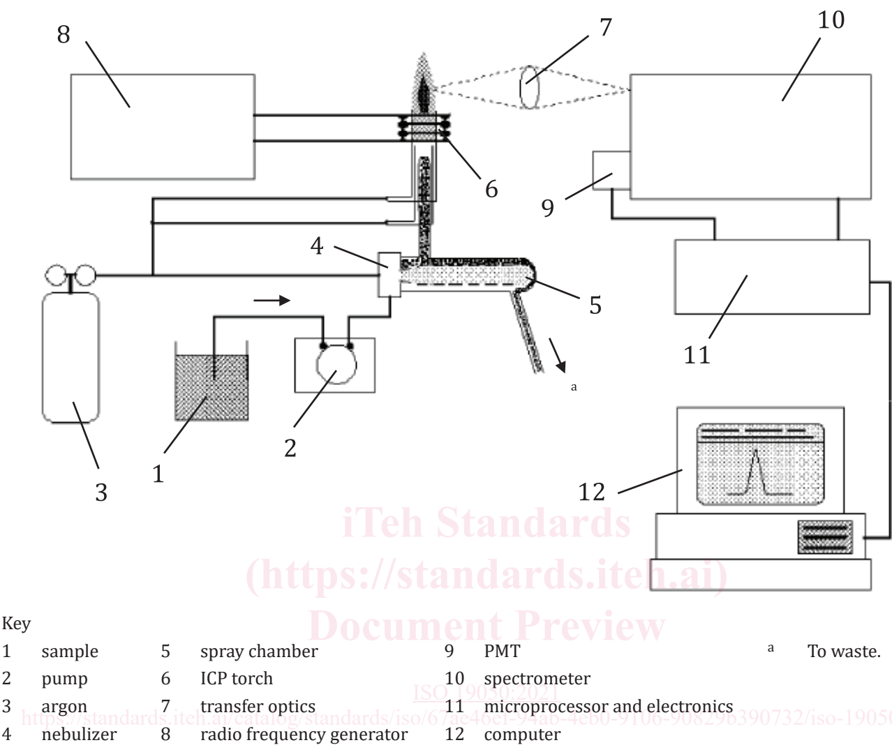
Figure 1 — Different components of a typical ICP-OES instrument
