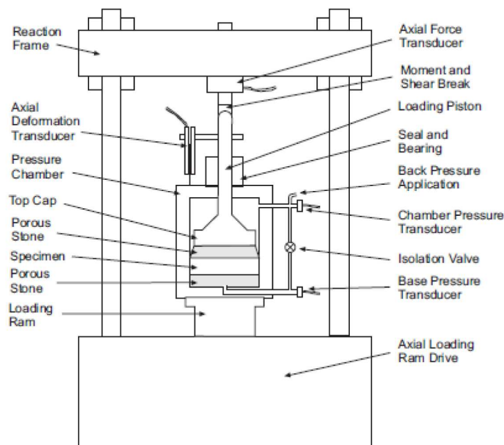
FIG. 1 Overview of Primary Components of a CRS Apparatus
