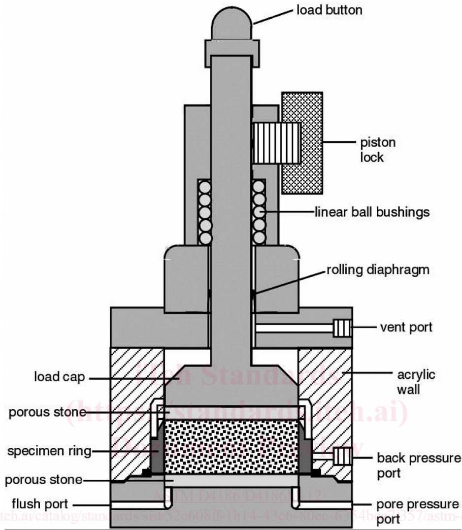
FIG. 42 Example of a CRS Consolidometer
