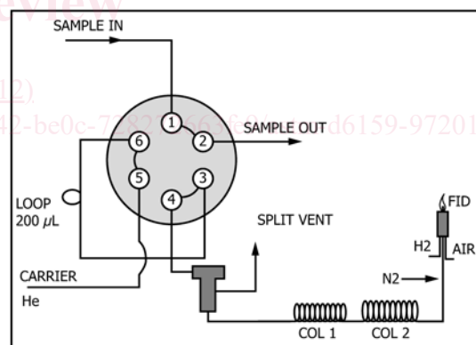
FIG. 4 Valve On – Injection
