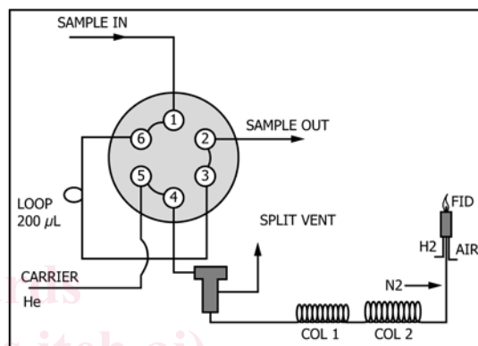
FIG. 3 Valve Off – Sample Loading
