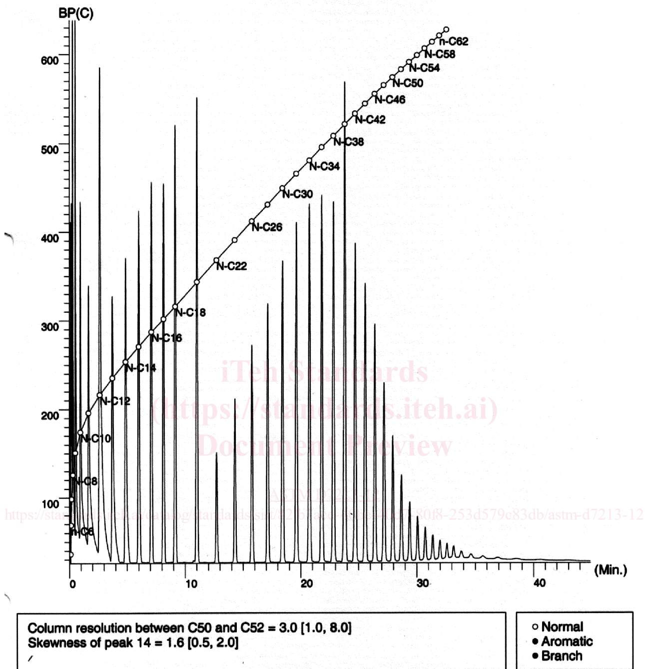
FIG. 1 Typical Calibration Curve with Plot
