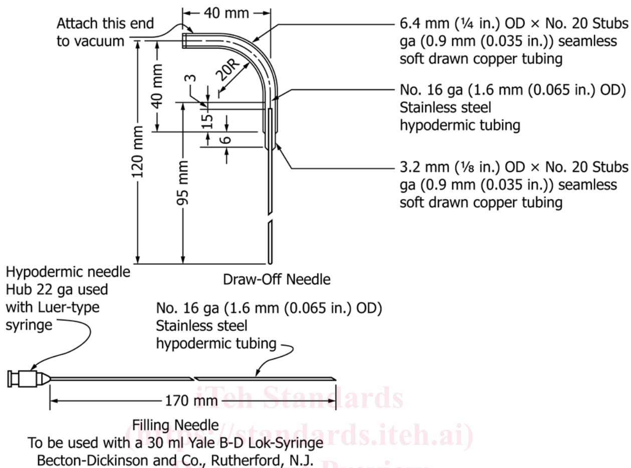
FIG. 3 Accessories for Bingham-Type Pycnometer
