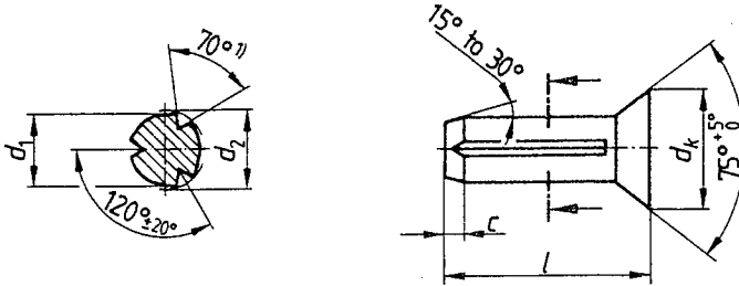
Type A Pin with chamfered end
