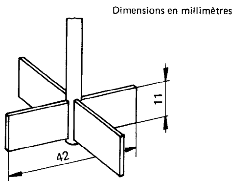
FIGURE — Agitateur
