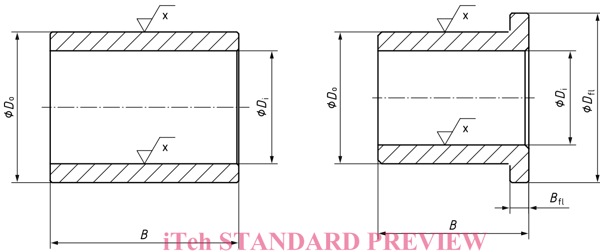
a) Cylindrical bush (standards.iteh.ai) b) Flanged bush
