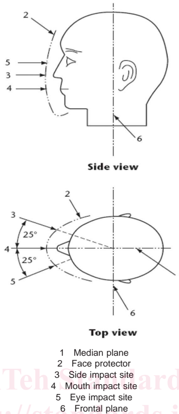
FIG. 2 Puck Impact Sites for Testing Face Protectors
