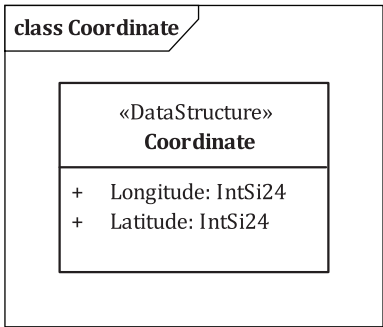
Figure 3 — Coordinate
