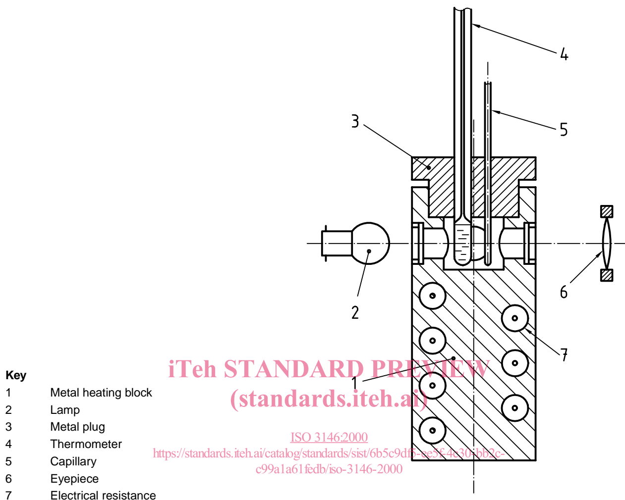
Figure 1 — Apparatus for method A
