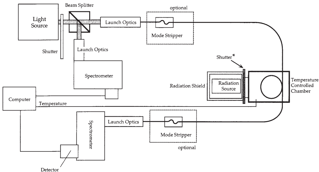
FIG. 1 Schematic Instrumentation Diagram
