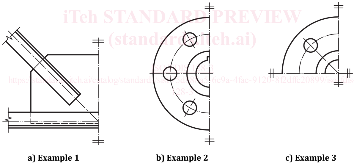
Figure 3 — Examples of simplified views of symmetrical parts
