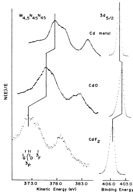
FIG. 1 Comparison of X-ray Excited Cd M 4,5 , N 45 , N 45 , 3d 5/2 Photoelectron Energy Shifts for Cd Metal, CdO, and CdF 2 (Ref. (1316))
