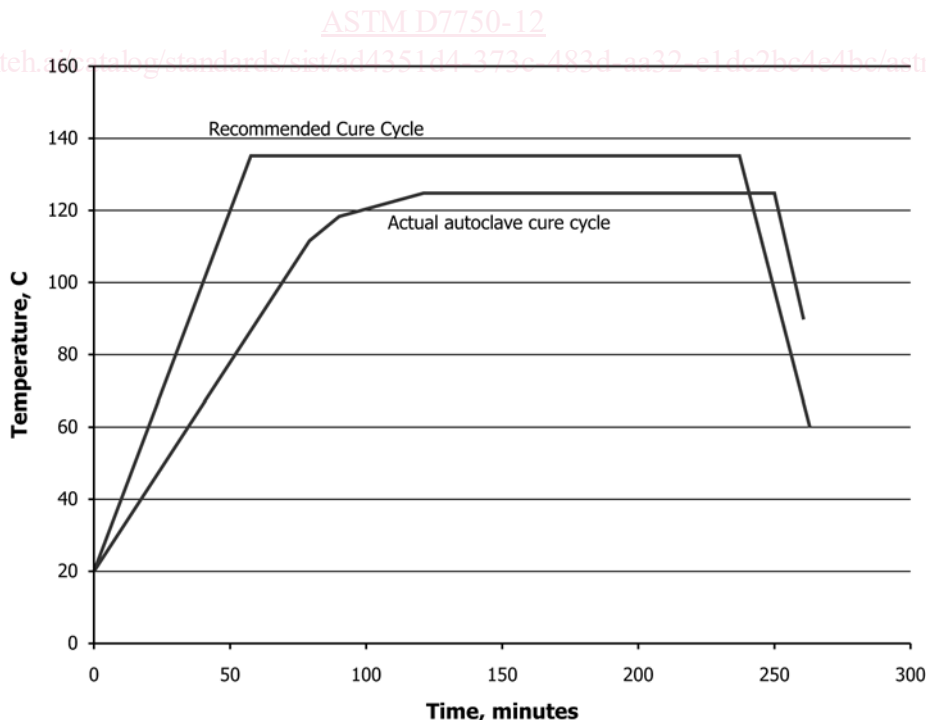
FIG. 2 Typical temperature program to cure components and the actual temperature at the component.
