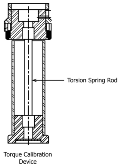
NOTE 1—Device is inserted between the plates when they are in the open position and the device is fastened to the upper and lower plates. FIG. 4 Typical Torque Standard used to calibrate the torque measurement system in an encapsulated specimen parallel plate rheometer.
