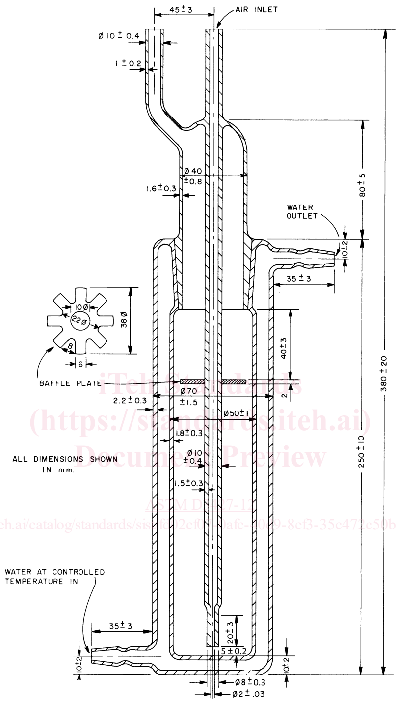
FIG. 2 Test Vessel
