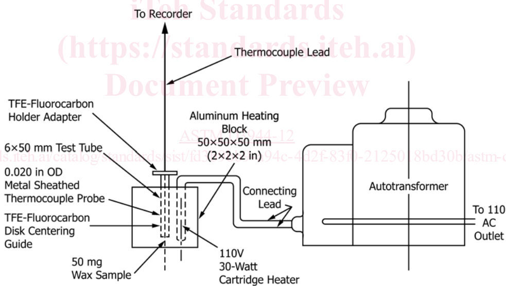
FIG. 2 Apparatus for Heating Wax Sample
