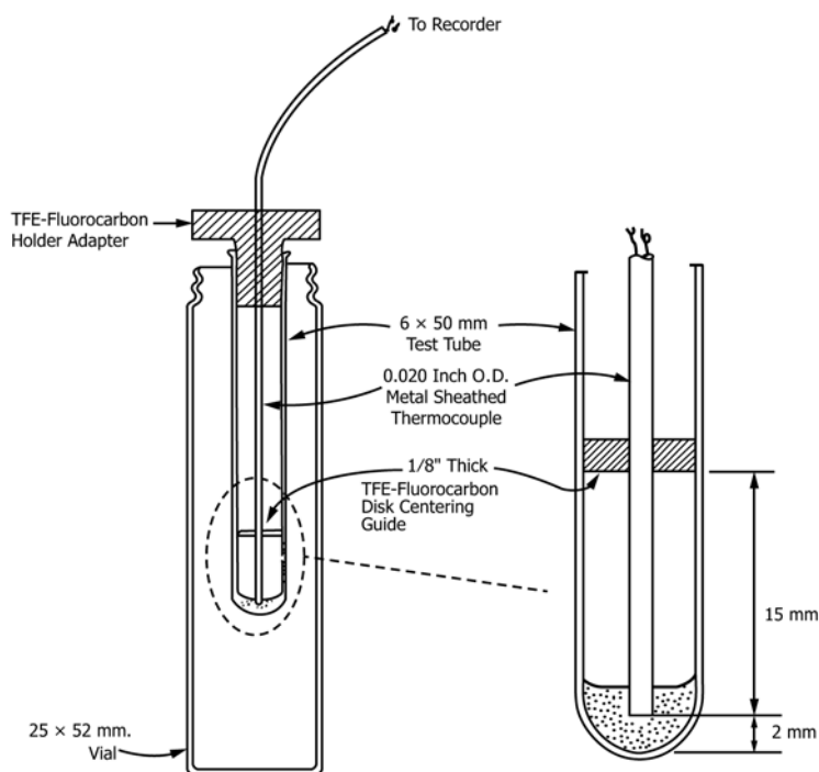
FIG. 1 Solidification Point Apparatus
