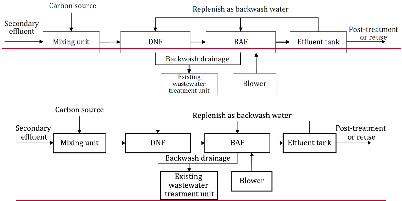
Figure 2 — Possible process flow diagram for applying biological filtration for total nitrogen removal from the secondary effluent containing \text{NH}_3\text{-N}
