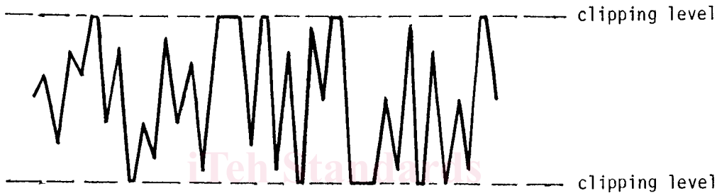
FIG. 3 Clipping of Fatigue Spectrum Loading
