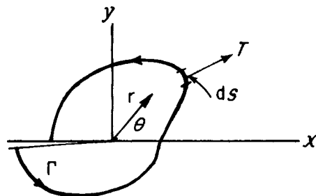
FIG. 2 J-Integral Crack Tip Contour and Symbolism for Path-Independent Crack Tip Integrals
