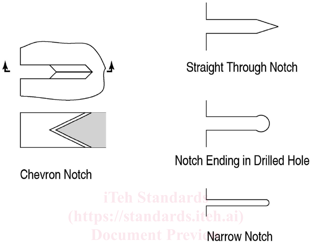
https://standards.itih.ai/catalog/standards/astm-e1921-13 FIG. 4 Envelope Crack Starter Notches 292-013a412bd0e0/astm-e1921-13
