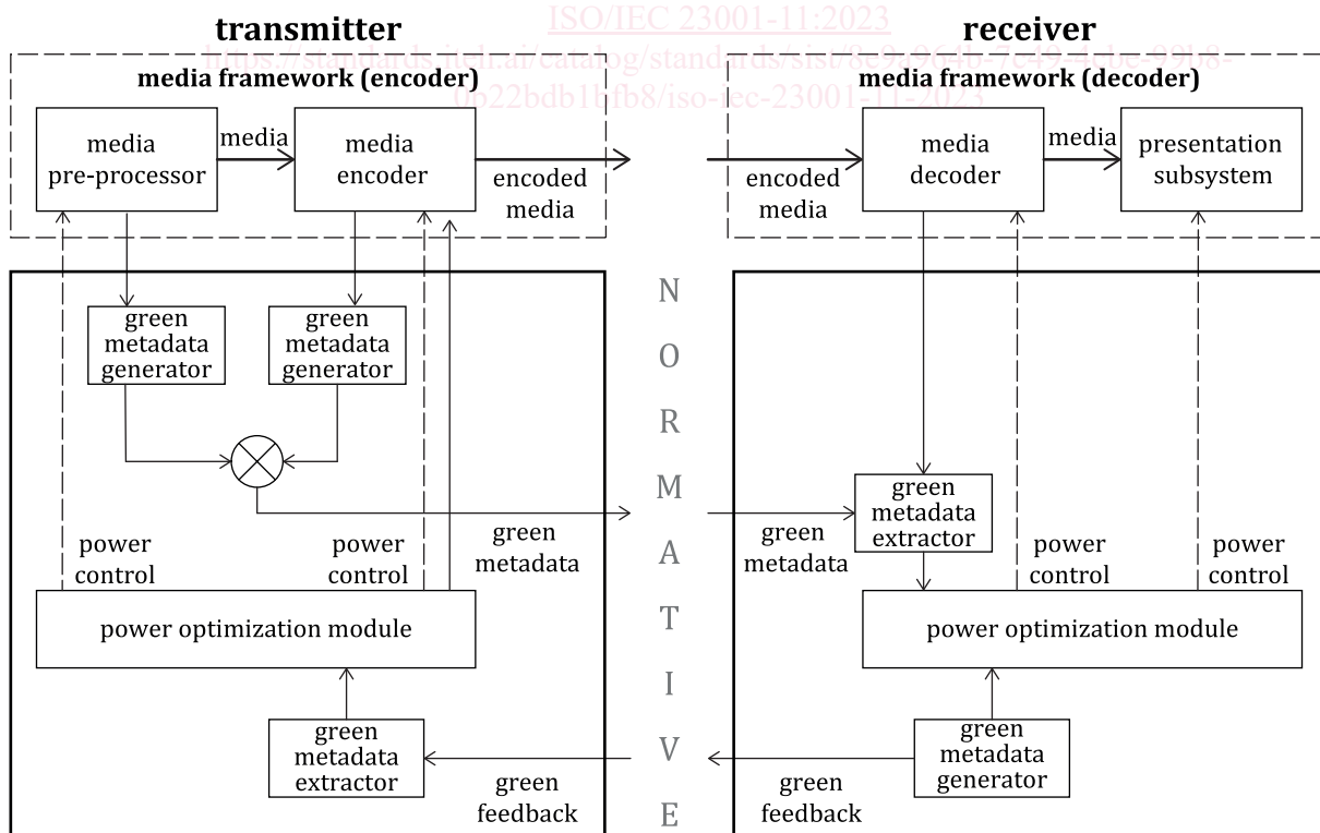
Figure 1 — Functional architecture
