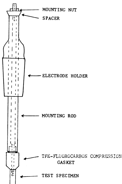
FIG. 54 Specimen Mounted on Electrode Holder
