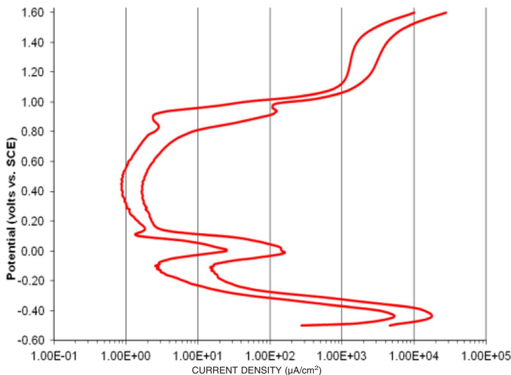
FIG. 21 Typical Standard Potentiodynamic Anodic Polarization Plot
