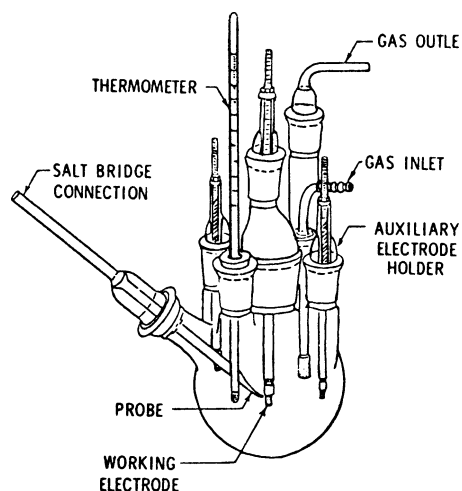
FIG. 32 Schematic Diagram of Polarization Cell (1)
