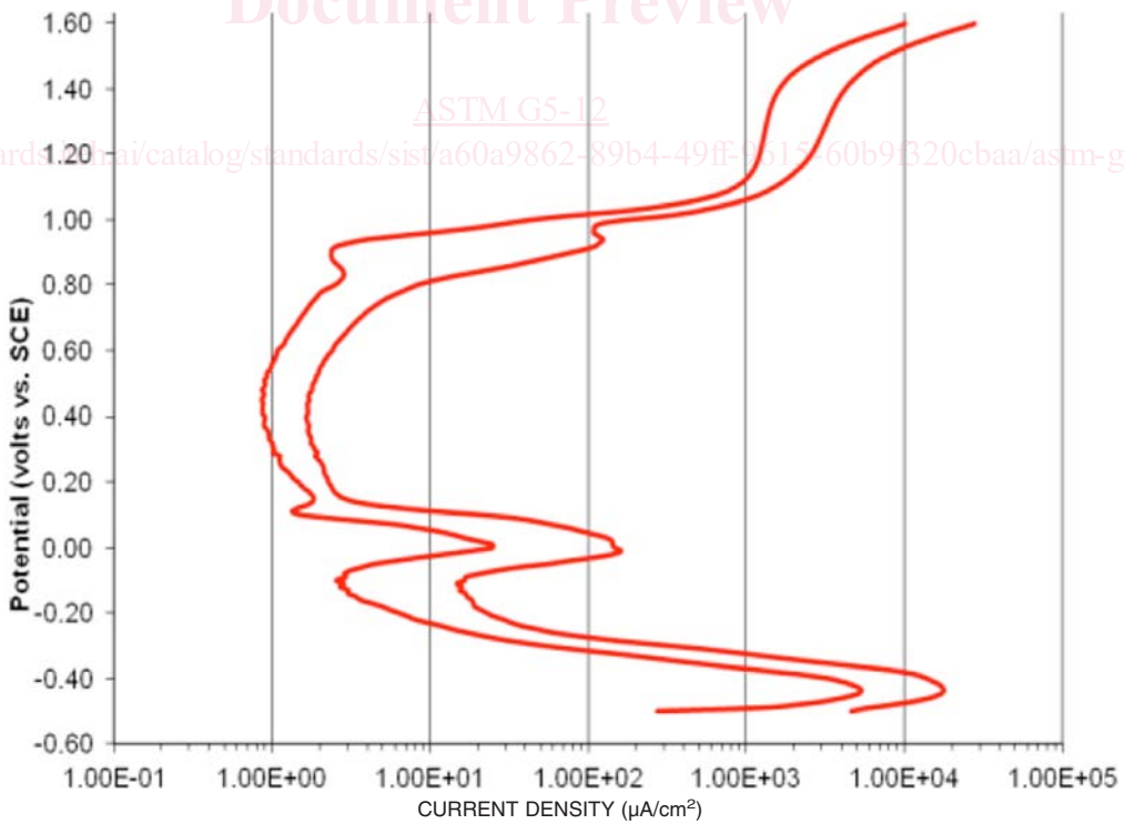
FIG. 2 Typical Standard Potentiodynamic Anodic Polarization Plot
