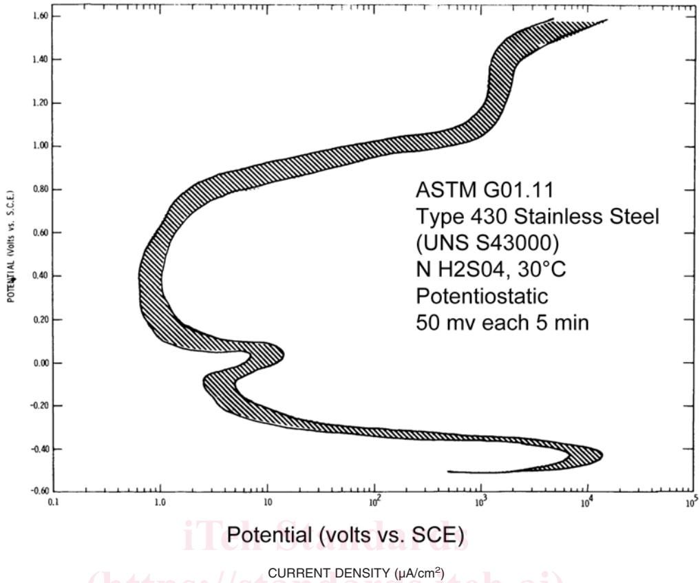
FIG. 1 Typical Standard Potentiostatic Anodic Polarization Plot
