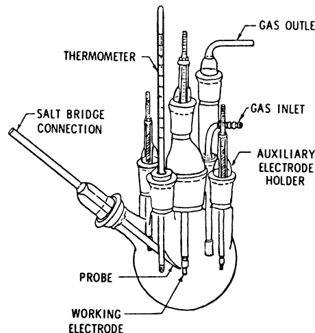
FIG. 3 Schematic Diagram of Polarization Cell (1)
