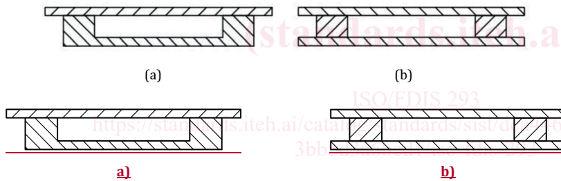
Figure_1 — Schematic diagram of flash mould (picture frame mould)
