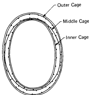
FIG. 3 Quadrant Reinforcement, Vertical Elliptical Pipe
