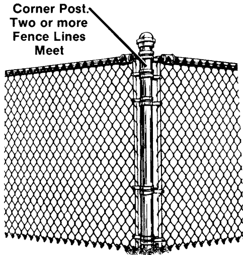
FIG. 2 Corner Post
